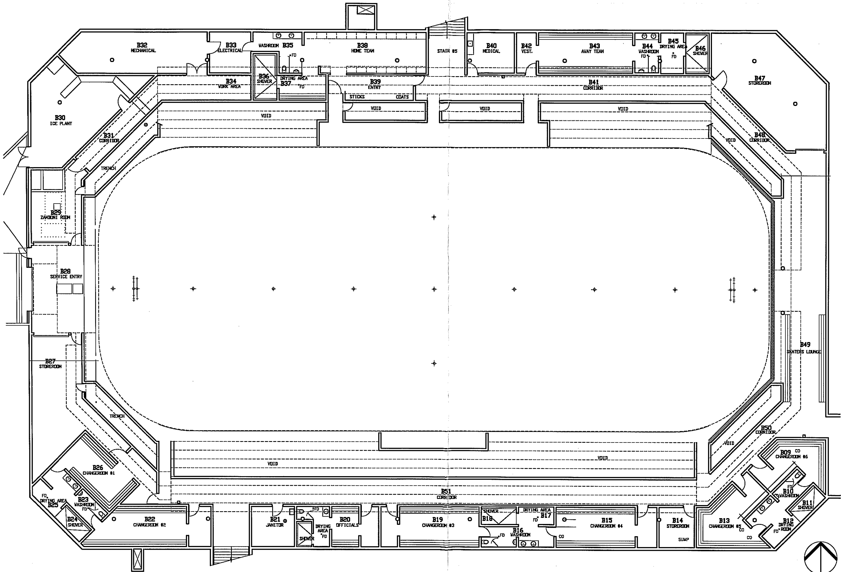
1 ARENA PLAN MAIN LEVEL 1:200
